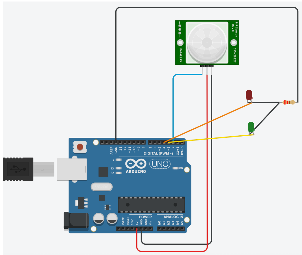
Figure 1. Schematic diagram of a PIR sensor with LED
